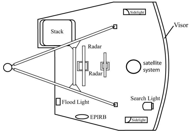
PILOTHOUSE TOP
