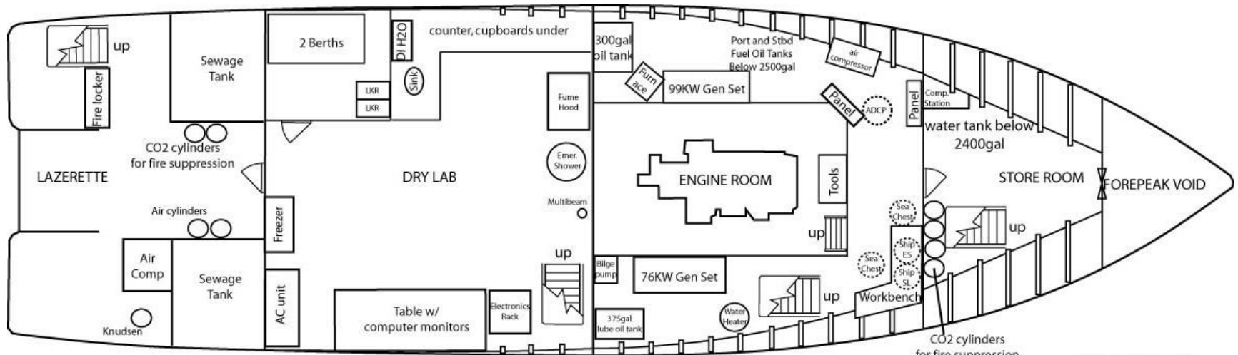
LOWER DECK
