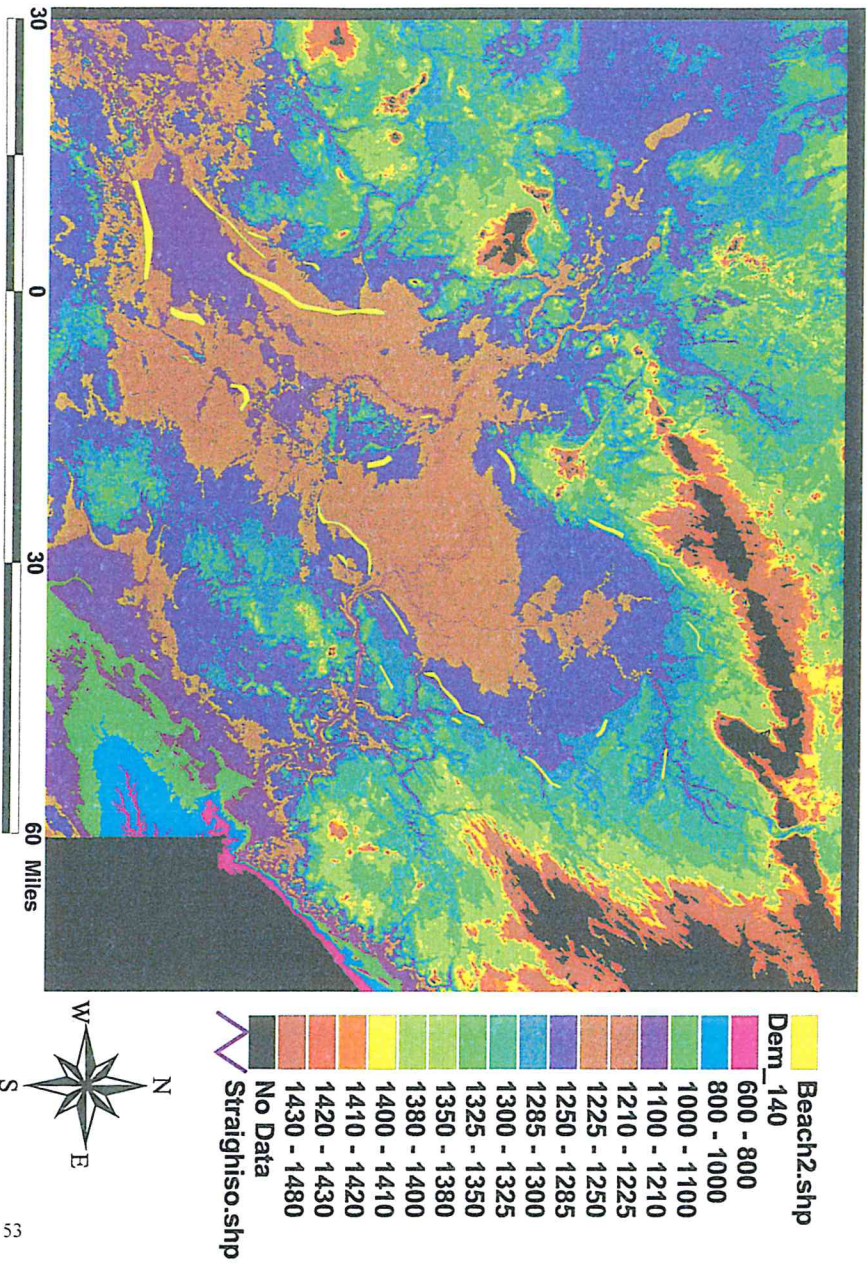
Figure 25h Digital Elevation Reconstruction of Lakes Atkin and Upham: 154 ft of uplift.
