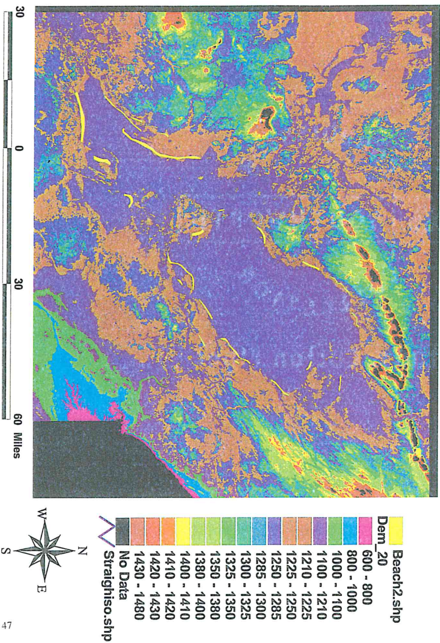
Figure 25b Digital Elevation Reconstruction of Lakes Aitkin and Upham, 22 ft of uplift.
