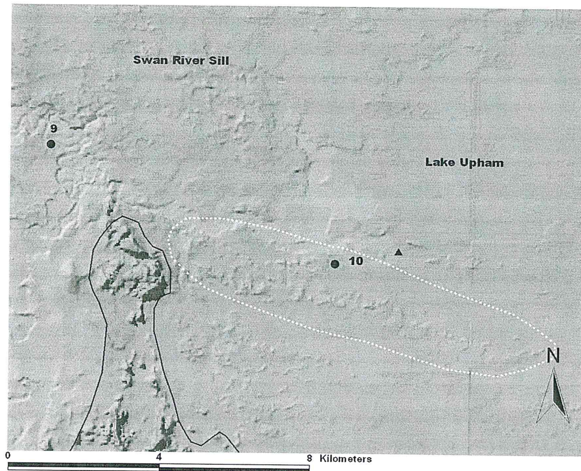
Fig 31. Ball Bluff Spit is within dashed line. Circle labeled 10 indicates where clay is overlain by 1 meter of underflow sands. Triangle indicates field site that was lake clay at the surface.
