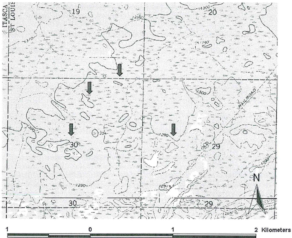
Figure 17. Dunes with respect to shore to basin contour lines (1300 and 1290 ft./ 396 m. and 393 m.), this is just northeast of the Swan River Sill in the Upham basin. Arrows are pointing to the dunes that are basinward of the 1300' and 1290' shoreline contour. (Floodwood 7.5 minute USGS quadrangle).
