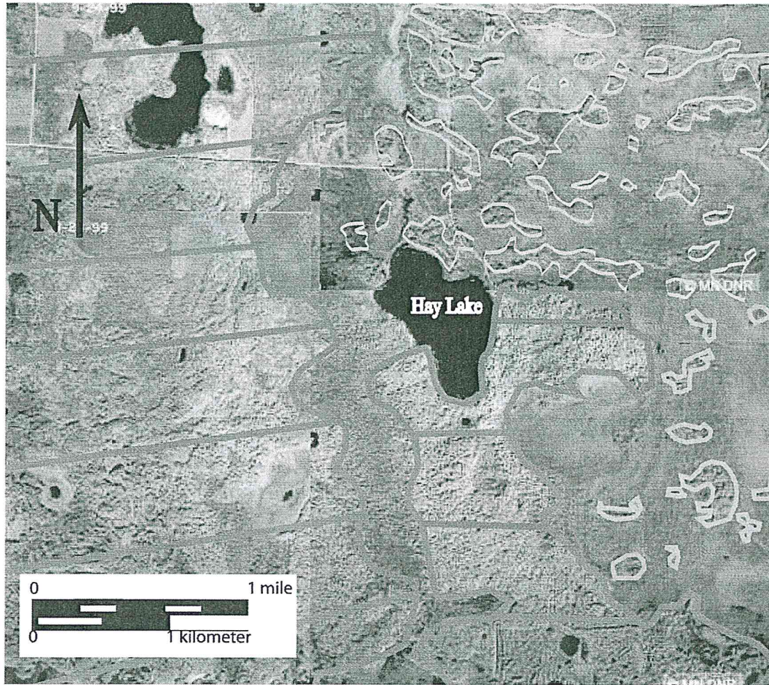
Figure 14. Aerial photo of Hay Lake. Horizontal lined areas indicate Lake Upham border; White polygons are dunes (Vanduse 7.5 minute USGS quadrangle).
