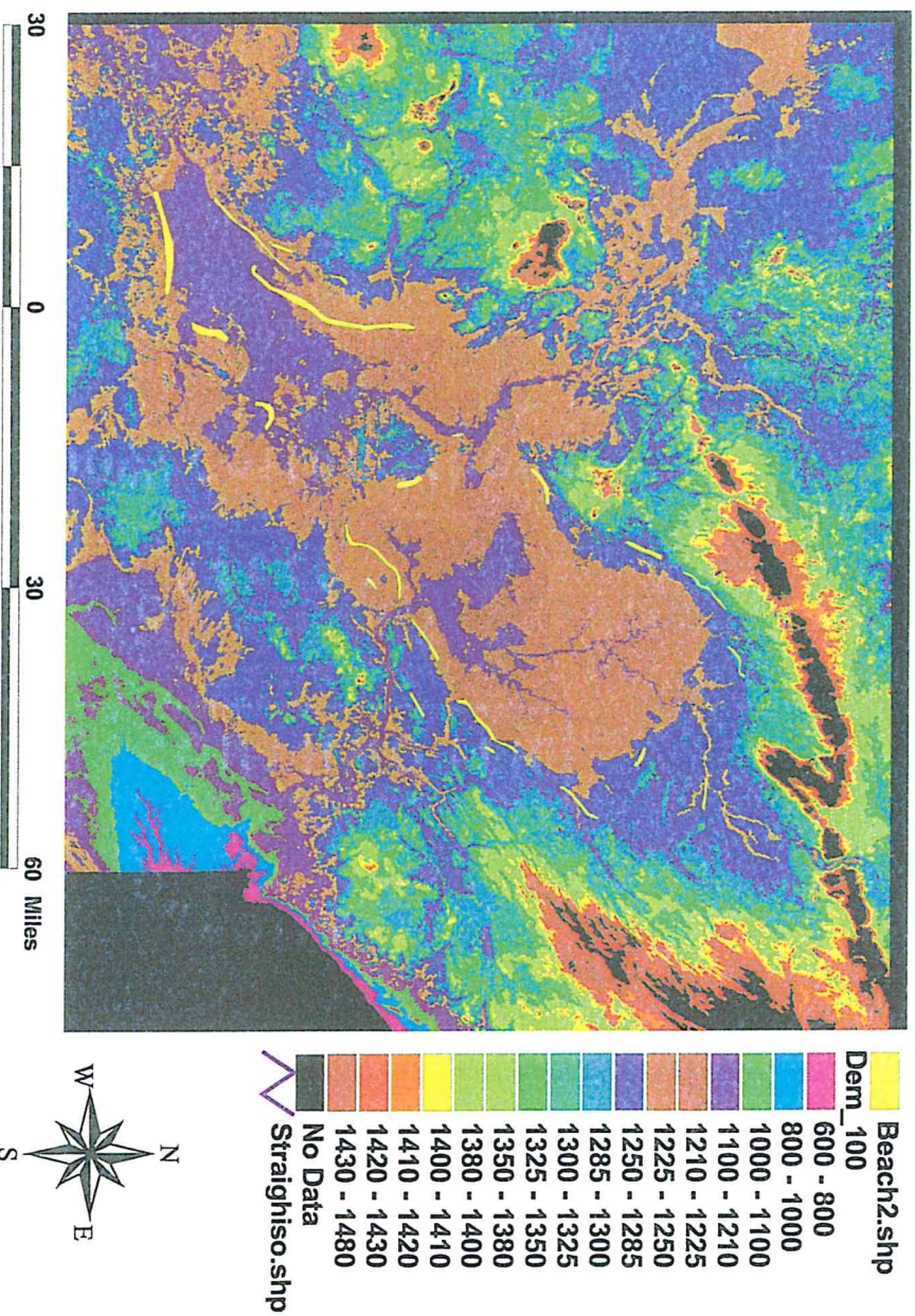
Figure 25f Digital Elevation Reconstruction of Lakes Aitkin and Upham, 110 ft of uplift.
