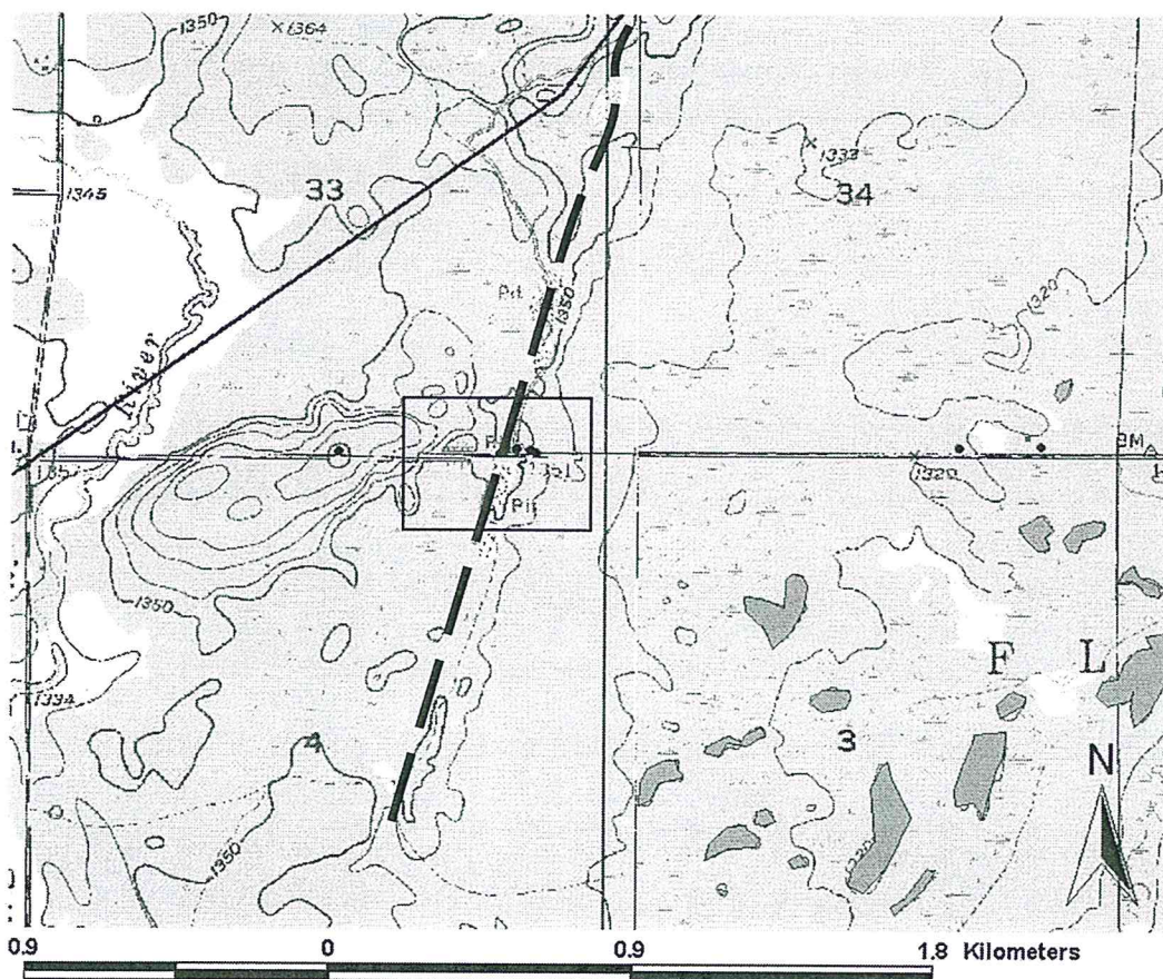
Figure 15. GPR survey along Lake Upham shoreline, marked by dots in the box. Dashed line is the border of Lake Upham. Polygons in southeast indicate dunes outlined in a colony (Silica and Riley 7.5 minute USGS quadrangle).
