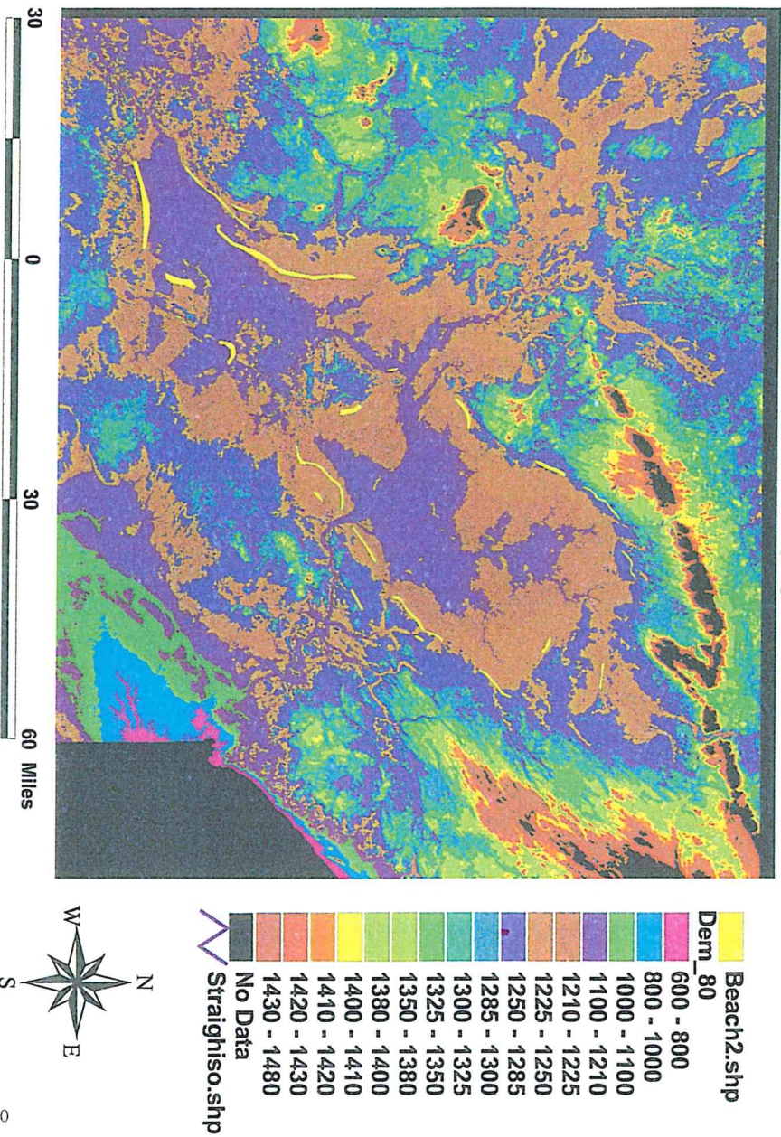
Figure 25c Digital Elevation Reconstruction of Lakes Atkin and Upham, 88 ft of uplift
