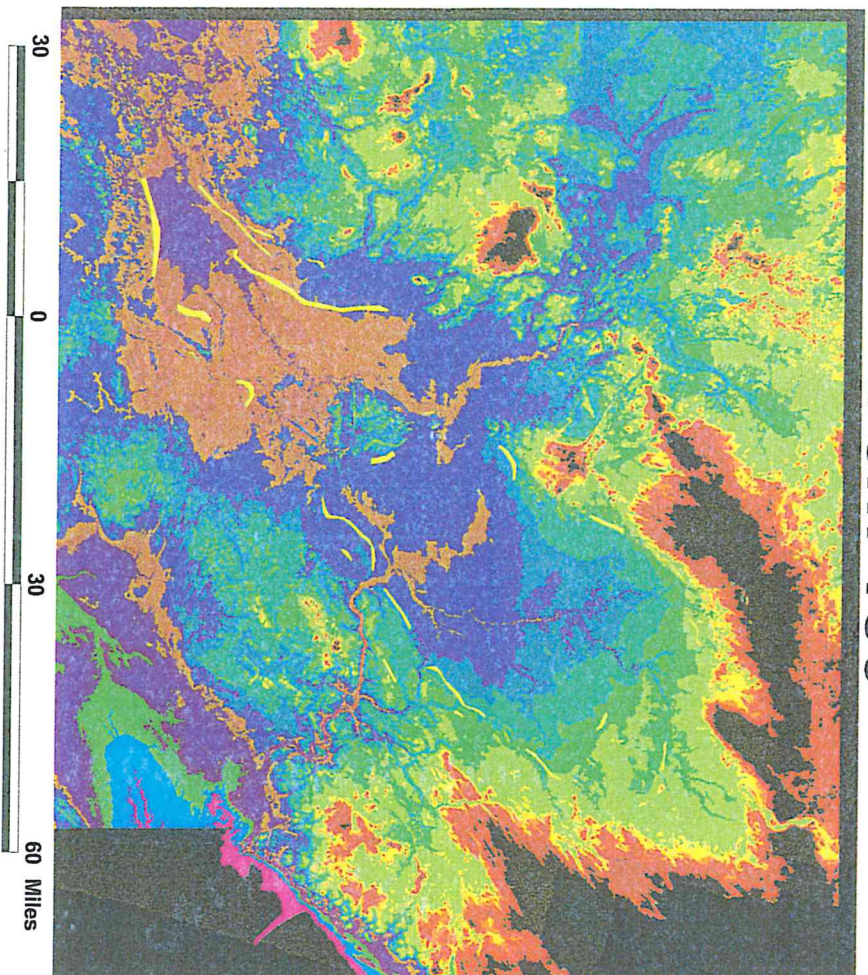
Figure 25j Digital Elevation Reconstruction of Lakes Aitkin and Upham, 198 ft of uplift.
