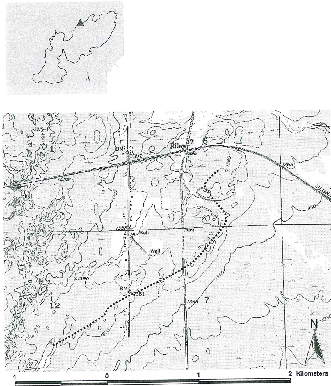
Figure 10. An example of a beach strandline (dashed line) in northern Lake Upham (Riley 7.5 minute USGS quadrangle).
