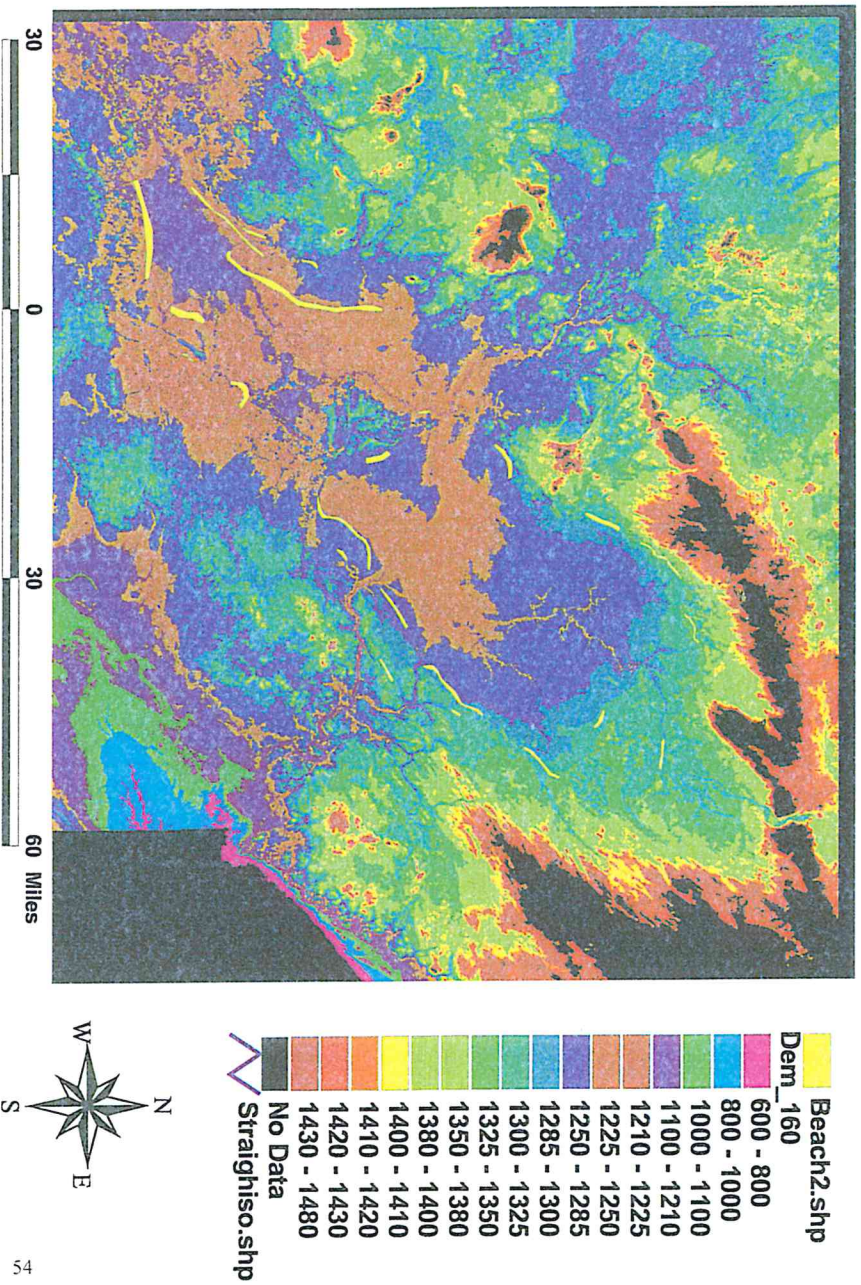
Figure 251 Digital Elevation Reconstruction of Lakes Atkin and Upham; 176 ft of uplift.
